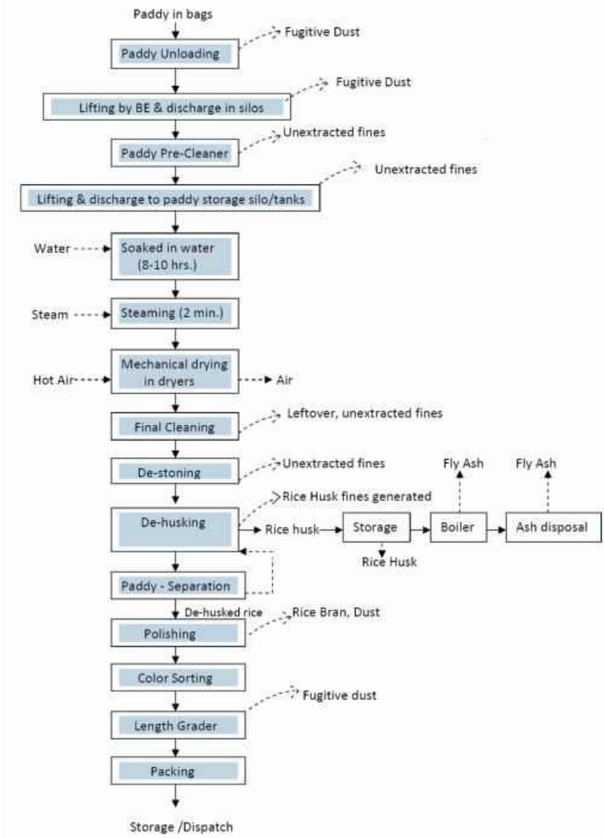
Fig 5.15-Typical Fugitive Emission Sources in Rice Mills
